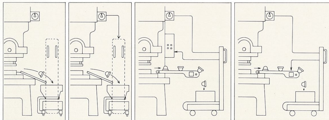
①センサ入力・シャッター連動 Sensor-shutter interlocking operation. ②カム入力・シャッター連動 Cam switch-shutter interlocking operation. ③カム入力・プレス連動 Cam switch-press interlocking operation. ④カム入力・コンベア連動 Cam switch-belt conveyor interlocking operation.
